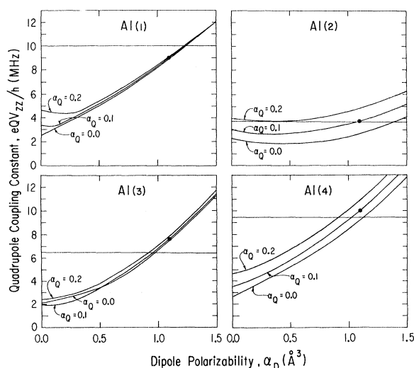
FIG. 1. Plot of the quadrupole coupling constants in kyanite vs the oxygen-ion dipolar polarizability. \alpha_Q is the quadrupolar polarizability. Horizontal line is the measured value. Large dot represents \alpha_D = 1.1 \text{\AA}^3 , \alpha_Q = 0.1 \text{\AA}^5 . Sternheimer factor = -2.6 .
